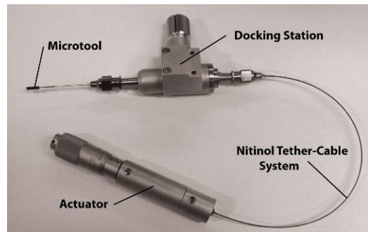
Fig. 4. Photograph of complete packaging and actuation system.
