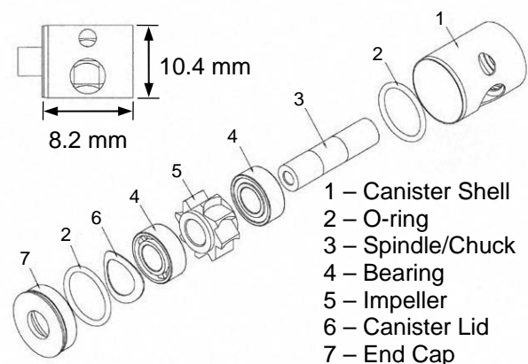
Figure 2. Exploded view of off-the-shelf dental drill air-turbine [excerpted from www.handpieceparts.com ]
