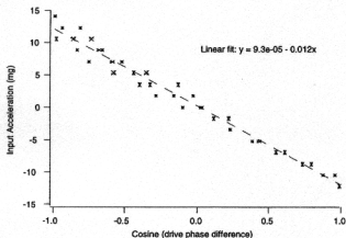
Figure 10. Closed loop scale factor test. Input acceleration nulled by adjusting phase between input drive voltages.
