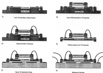
Figure 8. Micromachined POGA assembly procedure.
