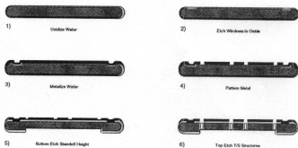
Figure 7. SDM/TSM assembly fabrication sequence.
