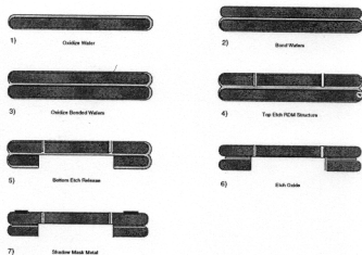
Figure 6. RDM fabrication sequence.
